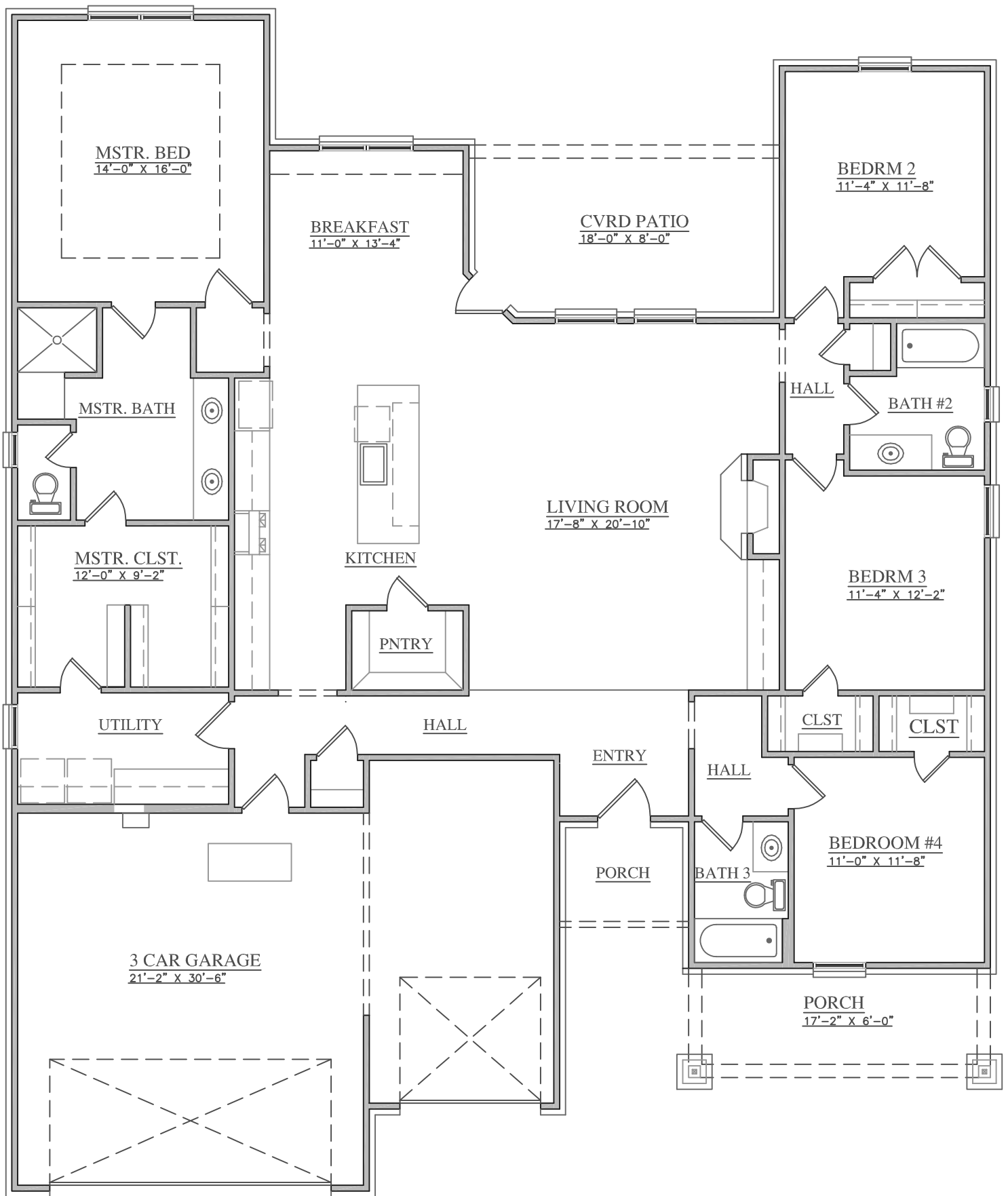
PLAN 2314
