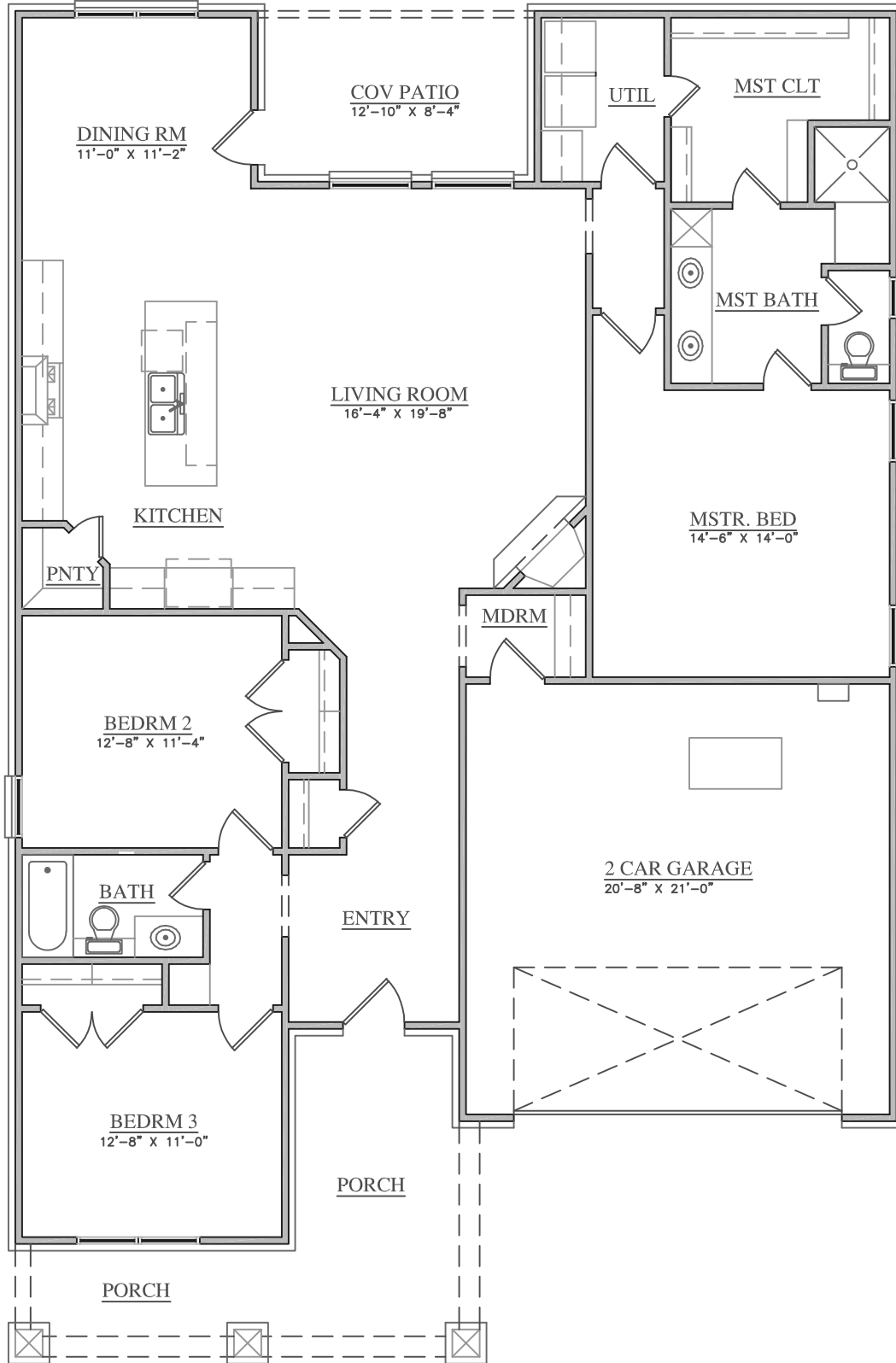
PLAN 1886
